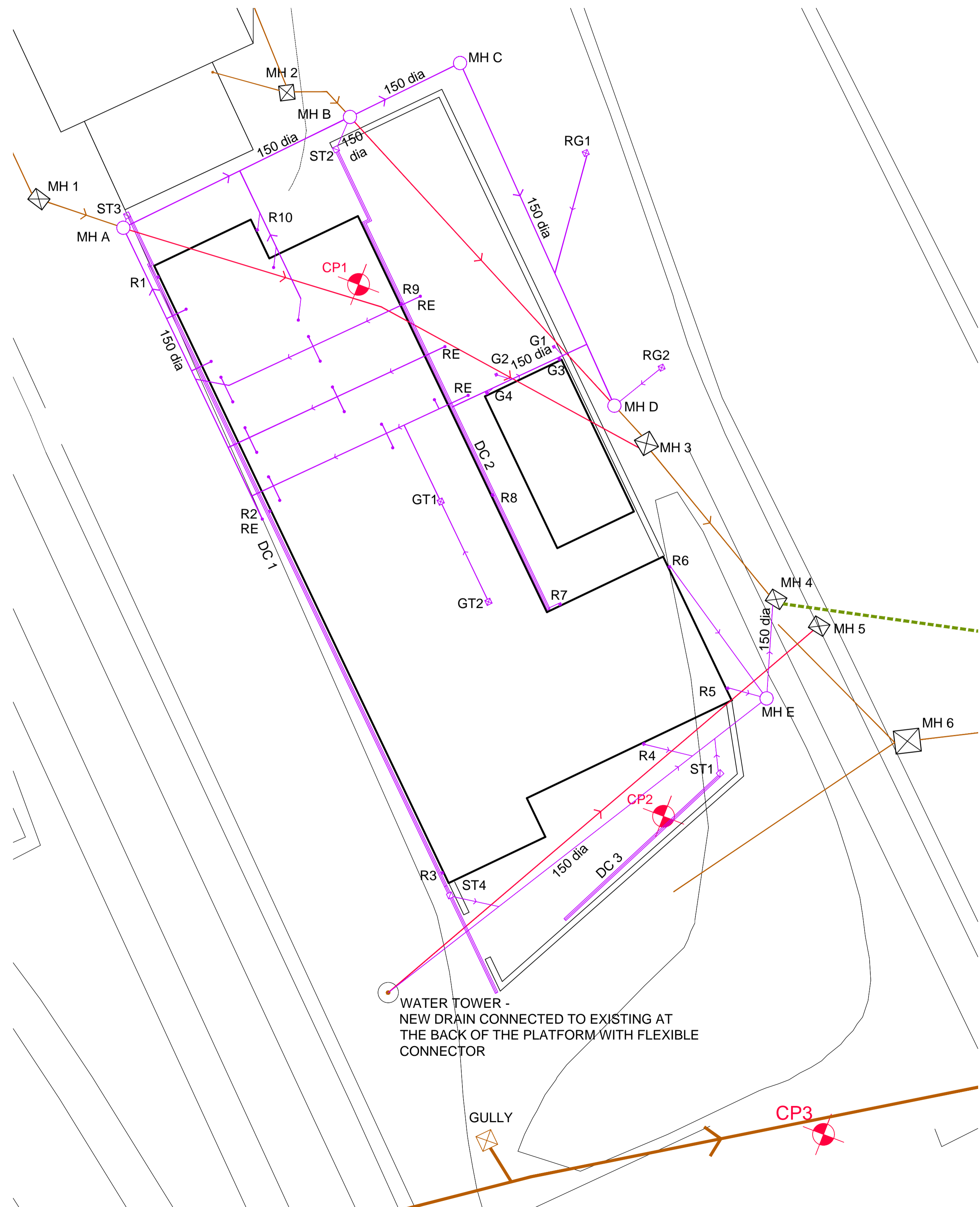
PROPOSED RESTAURANT DRAINAGE WORKS SCALE 1:100
